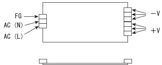
図6.5 -T1端子配列
