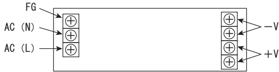
図5.3 -T端子配列
