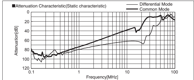
FSB-100-355
