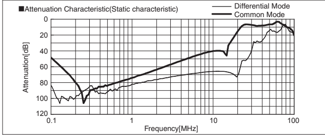
FSB-80-324
