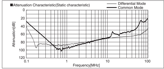
FSB-10-355
