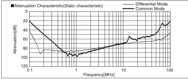
FSB-10-324
