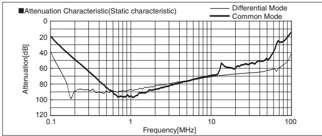
FSB-20-324
