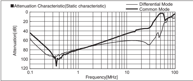
FSB-50-693-U
