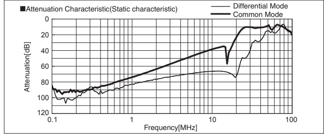
FSB-80-355
