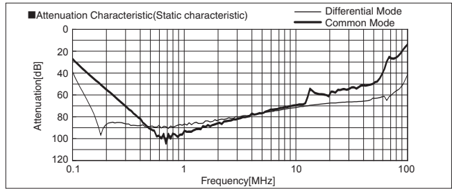
FSB-20-355
