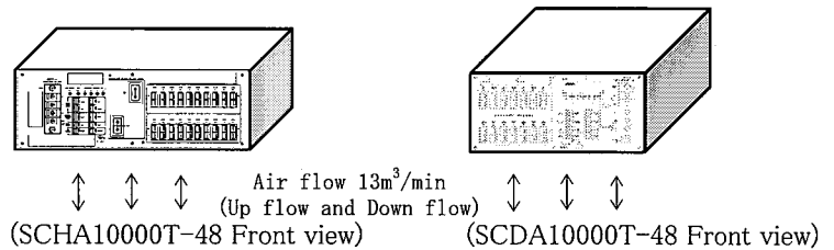
Mounting method(A)
