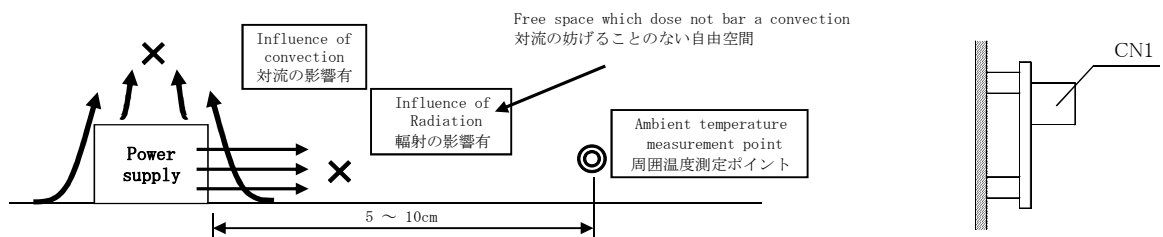
Mounting method (B)
