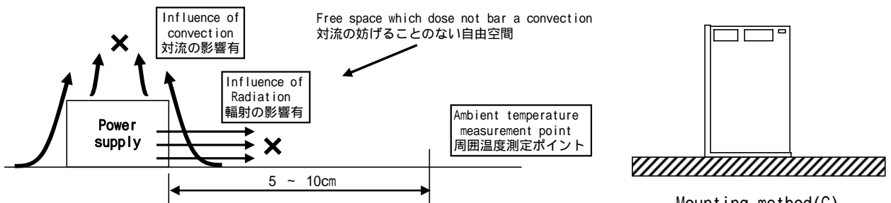
Mounting method(C)
