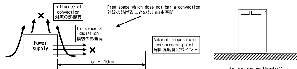
Mounting method(C)
