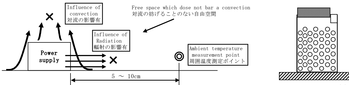
Mounting method (C)
