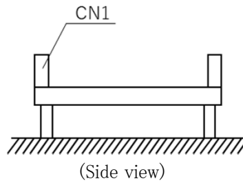
Fig.1.1 Mounting method (Normal position)
