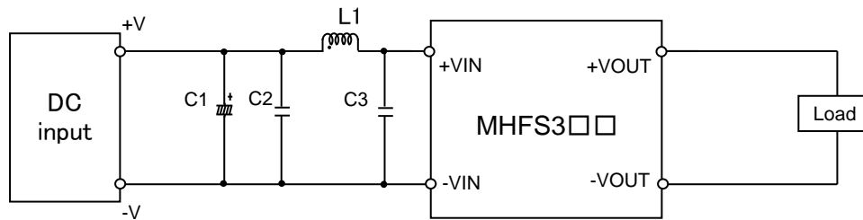
Fig.1 Testing circuitry
