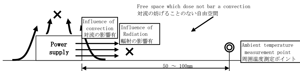
Mounting method(B)
