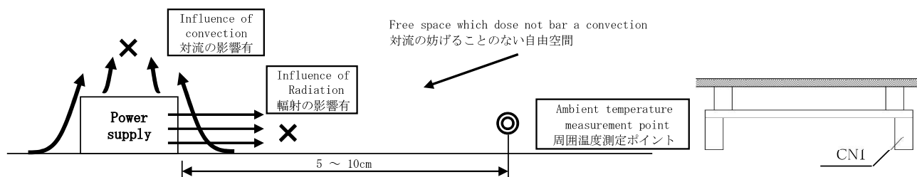
Mounting method (F)
