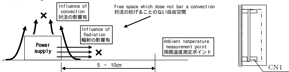
Mounting method(E)
