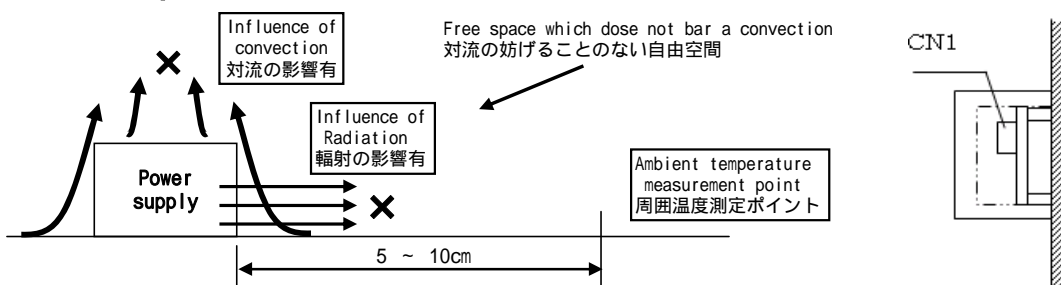
Mounting method(C)
