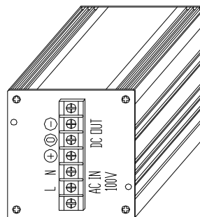
Mounting method(B)
