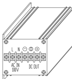
Mounting method(A)
