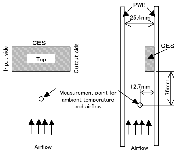
Fig1.1 Measuring method
