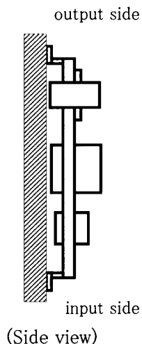
Fig.1.1 Mounting method
