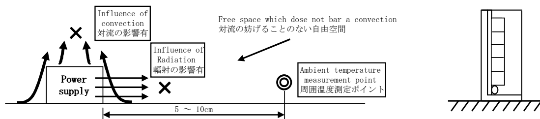
Mounting method(A)
