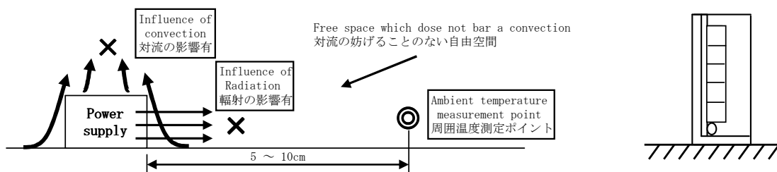
Mounting method(A)
