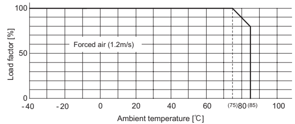
Fig.8.13 Derating curve (Forced air 1.2m/s)
