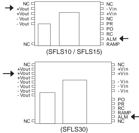
Fig.6.1 Measuring point
