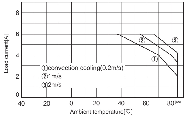
Fig.8.12 Load current vs. ambient temperature(CES48120-6 Vin=48V)
