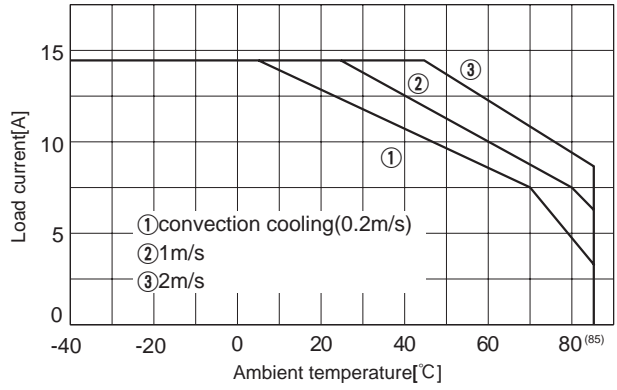
Fig.8.30 Load current vs. ambient temperature(CQS48120-14 Vin=48V)
