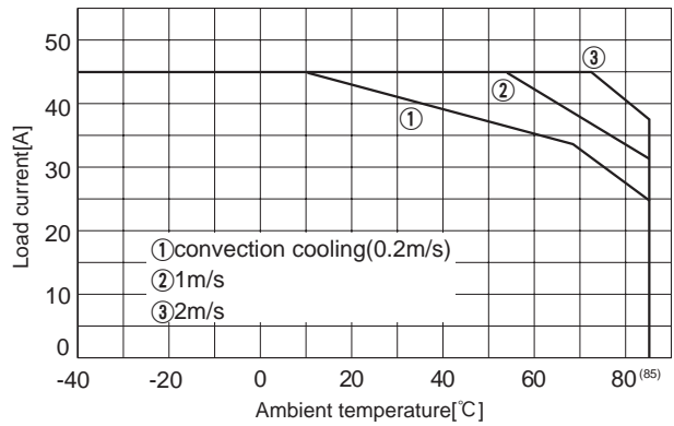
Fig.8.27 Load current vs. ambient temperature(CQS48025-45 Vin=48V)
