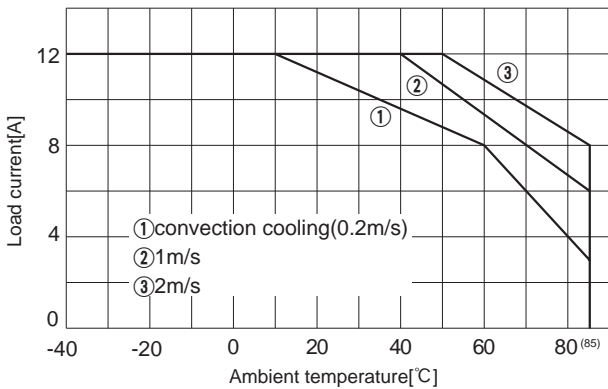
Fig.8.24 Load current vs. ambient temperature(CQS24120-12 Vin=24V)
