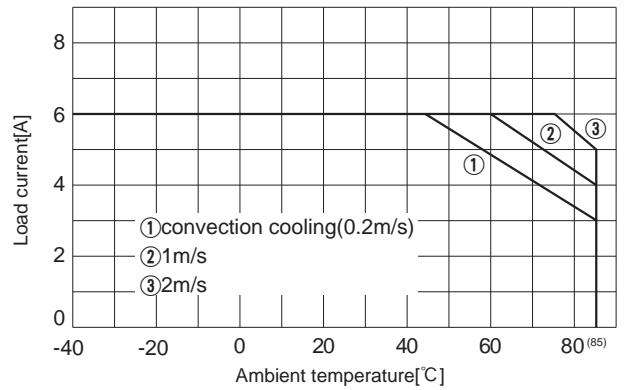
Fig.8.6 Load current vs. ambient temperature(CES24120-6 Vin=24V)
