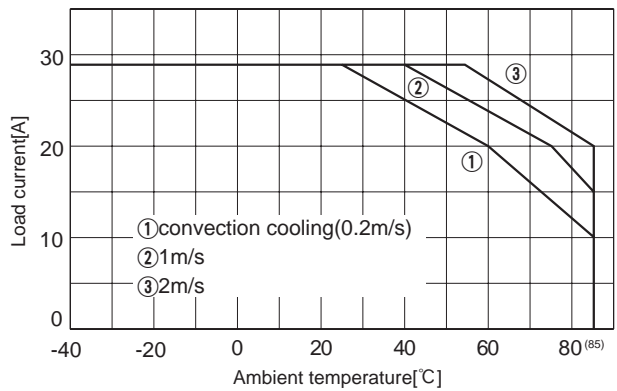
Fig.8.29 Load current vs. ambient temperature(CQS48050-28 Vin=48V)
