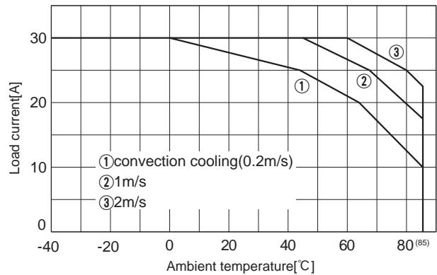
Fig.8.13 Load current vs. ambient temperature(CES48033-30 Vin=48V)
