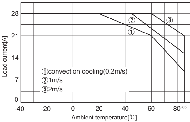
Fig.8.23 Load current vs. ambient temperature(CQS24050-28 Vin=24V)
