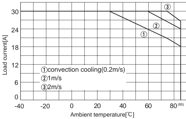
Fig.8.8 Load current vs. ambient temperature(CES48018-30 Vin=48V)
