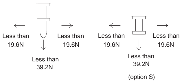
Fig.6.4 Stress onto the pins
