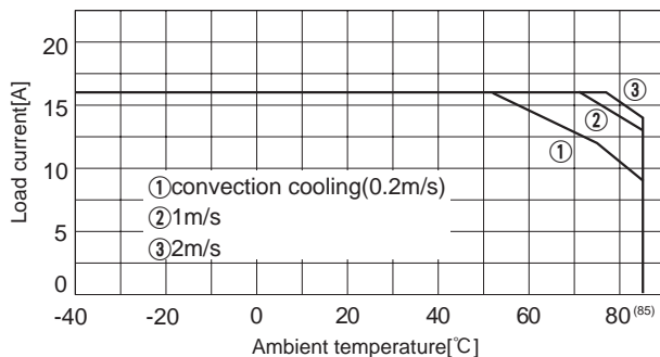
Fig.8.11 Load current vs. ambient temperature(CES48050-16 Vin=48V)
