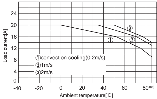
Fig.8.14 Load current vs. ambient temperature(CES48050-20 Vin=48V)
