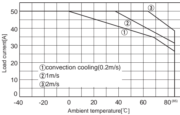
Fig.8.25 Load current vs. ambient temperature(CQS48015-50 Vin=48V)
