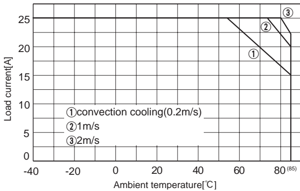
Fig.8.9 Load current vs. ambient temperature(CES48025-25 Vin=48V)
