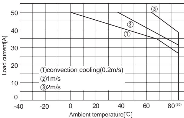
Fig.8.26 Load current vs. ambient temperature(CQS48018-50 Vin=48V)
