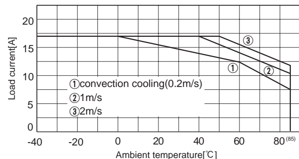
Fig.8.15 Load current vs. ambient temperature(CES48060-17 Vin=48V)
