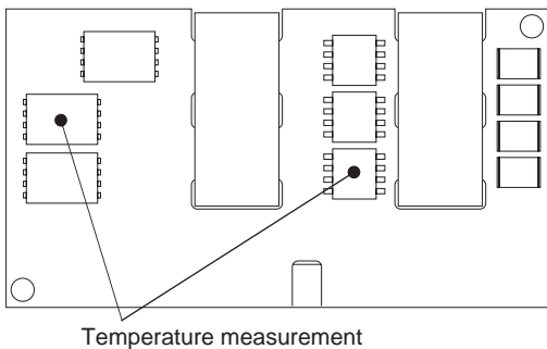
Fig.8.19 CQS48050-28, Temperature measurement location
