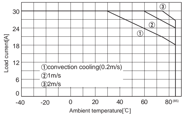
Fig.8.7 Load current vs. ambient temperature(CES48015-30 Vin=48V)
