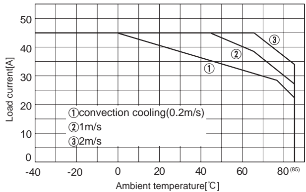
Fig.8.28 Load current vs. ambient temperature(CQS48033-45 Vin=48V)
