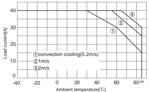
Fig.8.22 Load current vs. ambient temperature (CQS24033-40 Vin=24V)
