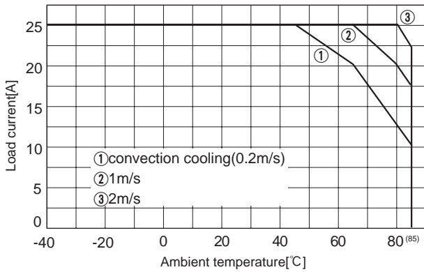
Fig.8.10 Load current vs. ambient temperature(CES48033-25 Vin=48V)
