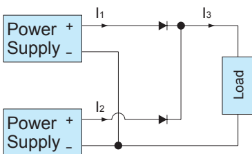
Fig.4.2 Redundancy operation
