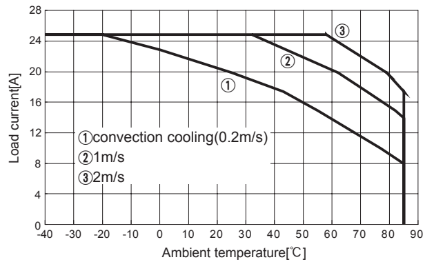
Fig.8.21 Load current vs. ambient temperature(CHS3004812H Vin=48V)
