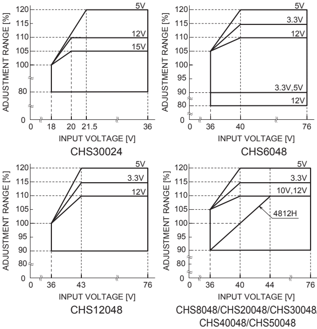
Fig.4.7 CHS Output Voltage Adjustment Range
