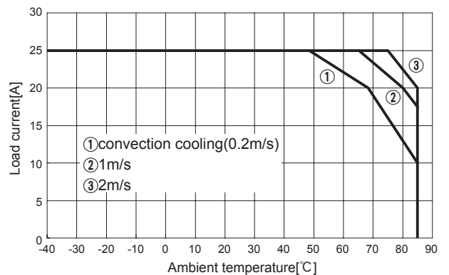
Fig.8.7 Load current vs. ambient temperature(CHS80483R3 Vin=48V)
