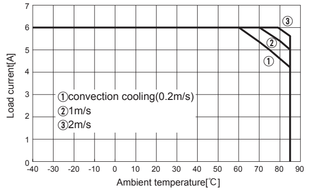
Fig.8.6 Load current vs. ambient temperature(CHS604812 Vin=48V)
