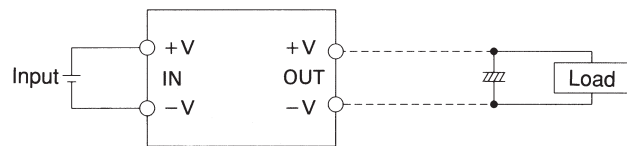
Fig.3.3 Connection method of capacitor at load
