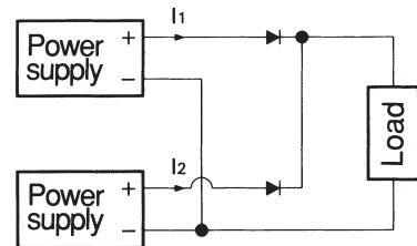
Fig.4.2 Redundancy operation
