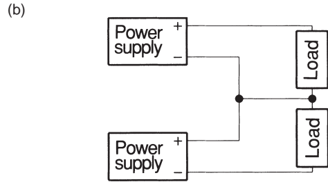
Fig.4.1 Series operation
