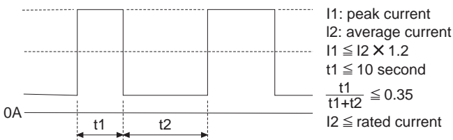
Fig.2.1 Peak current
