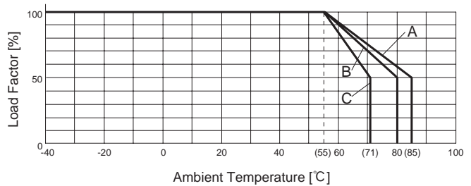
Fig.8.2 Derating Curve for Forced Air Cooling (1m/s) (SU/SUC1R5)
