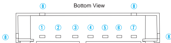
Fig.1.2 Pin Terminal Configuration
