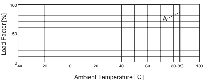
Fig.8.1 Derating Curve for Convection Cooling (SU/SUC1R5)
