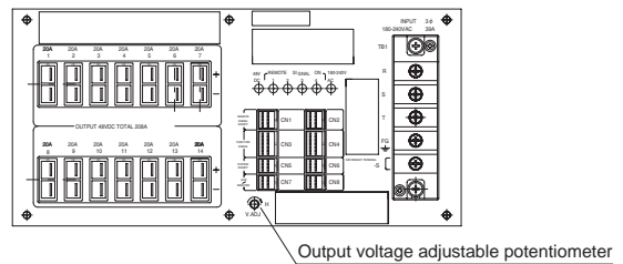
Fig.1.3 SCDA10000T Output voltage adjustable potentiometer
