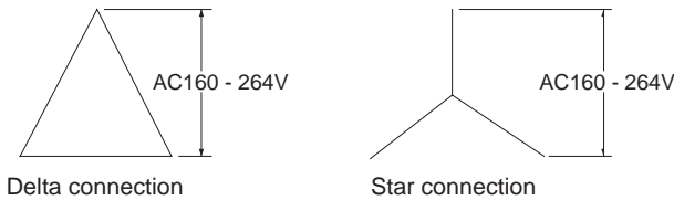
Fig.1.1 Connection method
