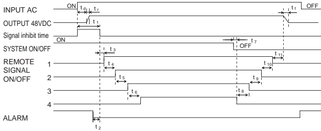
Fig.1.7 Timing diagram 1
