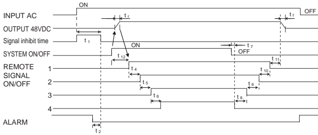
Fig.1.8 Timing diagram 2
