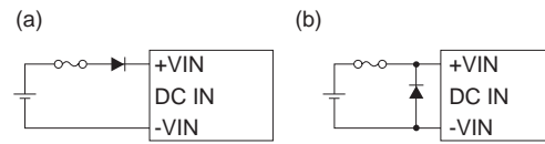
Fig.3.3 Reverse Input Voltage Protection
