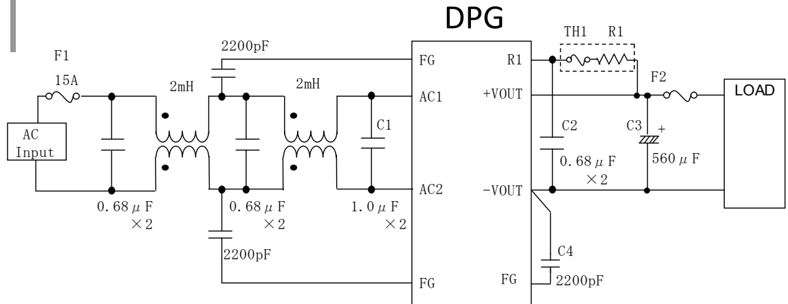
Fig.3.1 Recommended filter for DPG
