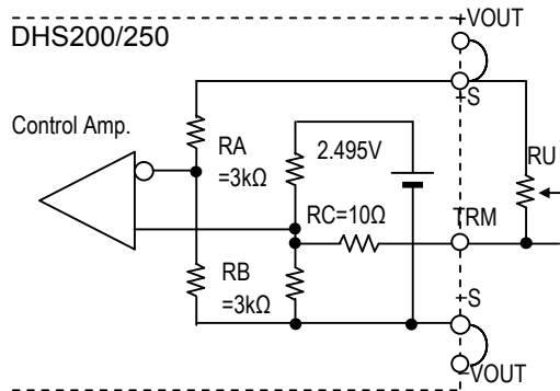
Fig. 5.6 Output voltage control circuit
