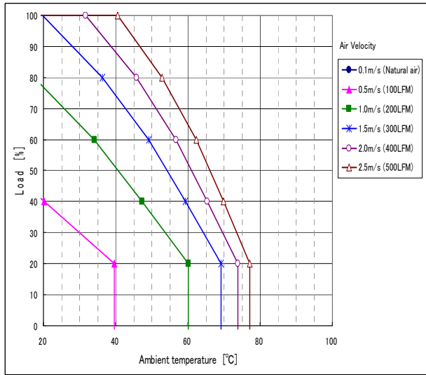
F-CBS-F1/F2 (H = 12.7mm)
