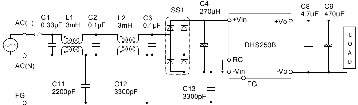
Fig. 10.5 Recommended circuit and noise level CISPR Pub.22 Class A)
