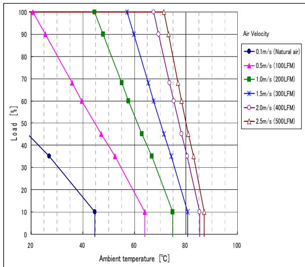
F-QB-F3/F4 (H = 25.4mm)
