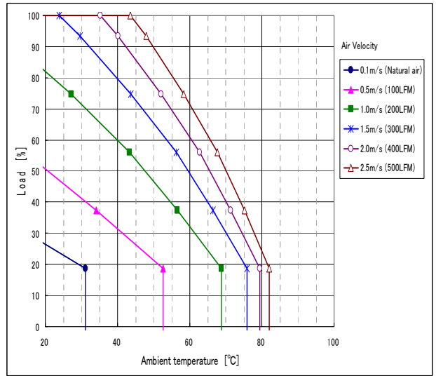
F-CBS-F1/F2 (H = 12.7mm)
