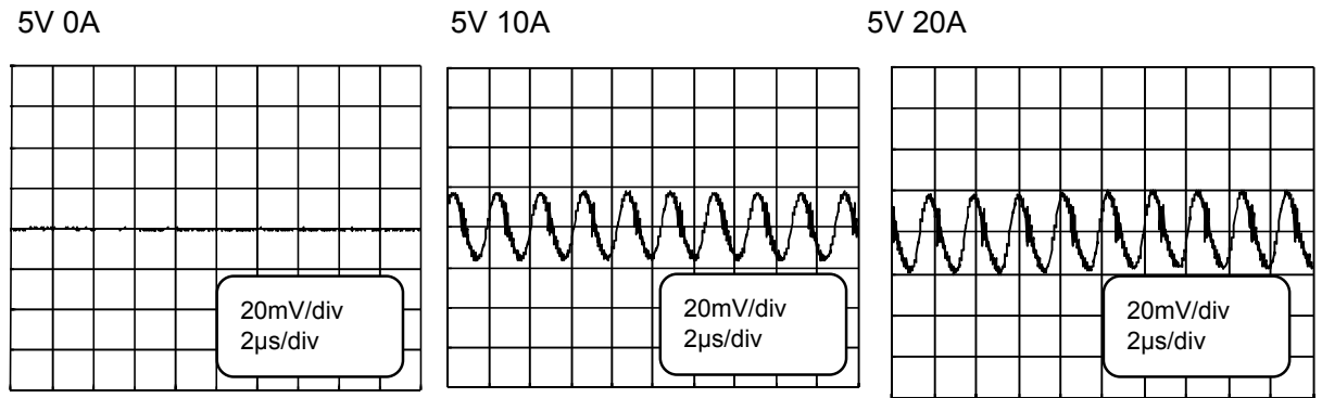
Fig. 10.9 Output noise
