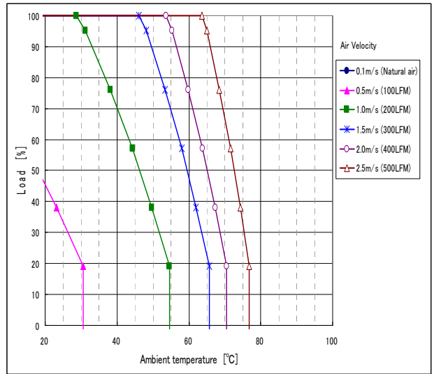
F-QB-F1/F2 (H = 12.7mm)
