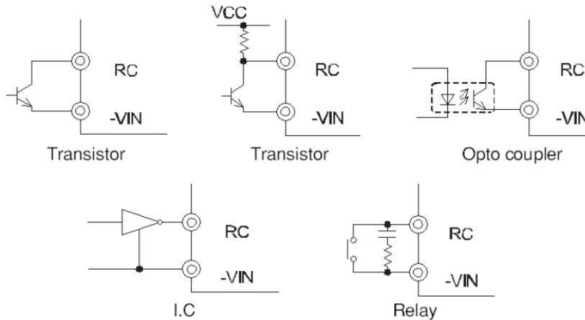
Fig. 6.2 RC connection example
