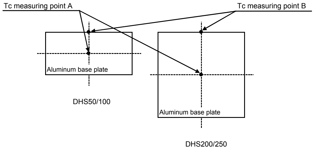
Fig. 11.2 Measuring point
