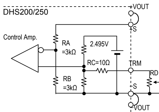
Fig. 5.5 Output voltage control circuit
