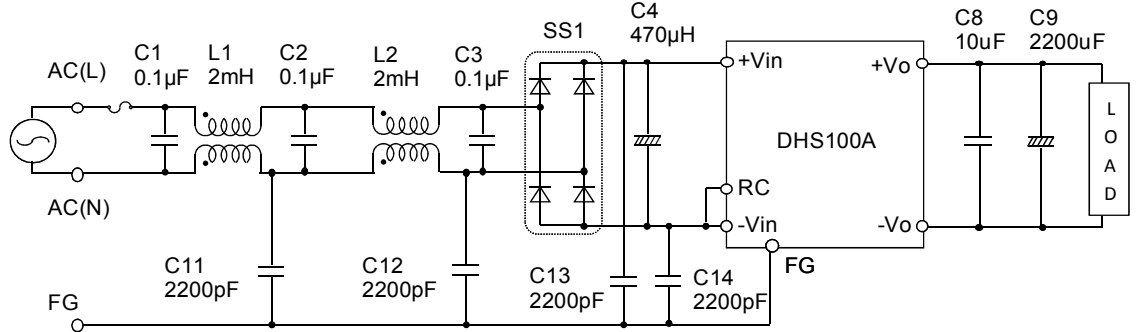
Fig. 10.3 Recommended circuit and noise level CISPR Pub.22 Class A)
