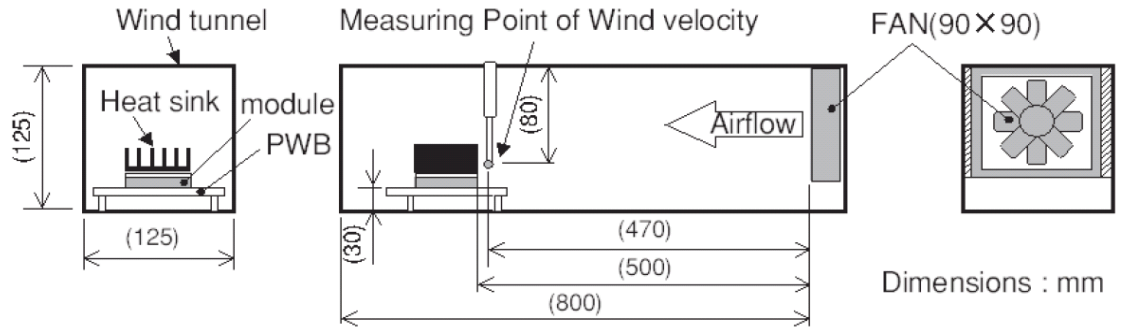
Fig. 12.1 Measuring environment
