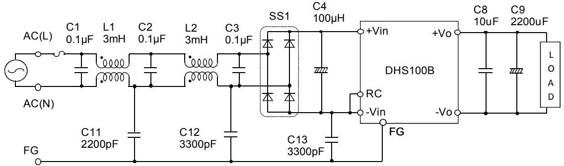
Fig. 10.4 Recommended circuit and noise level CISPR Pub.22 Class A)
