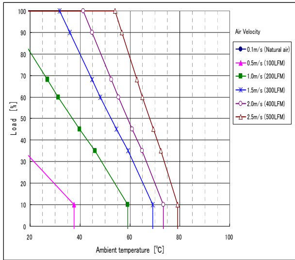
F-QB-F1/F2 (H = 12.7mm)
