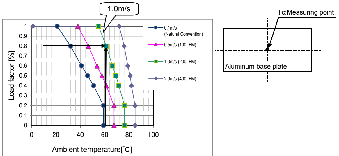
Fig. 12.3 Example of Thermal curves
