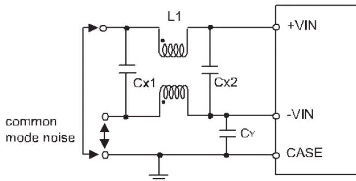
Fig. 10.1 Common mode noise path
