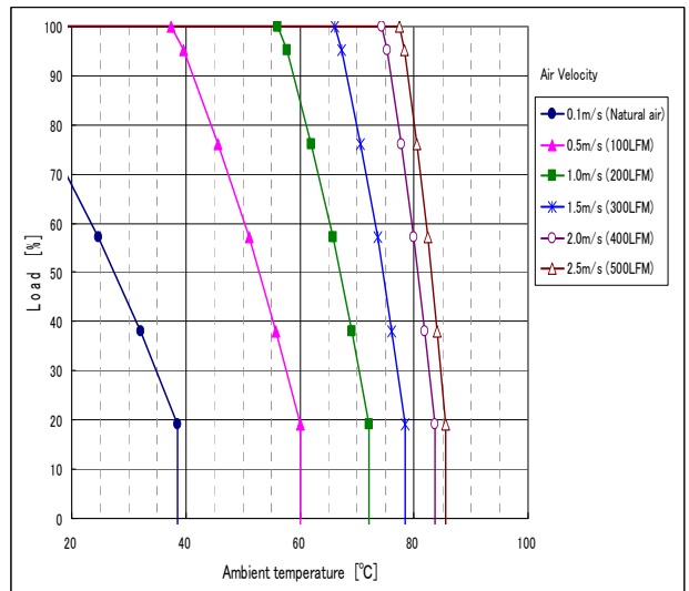
F-QB-F3/F4 (H = 25.4mm)
