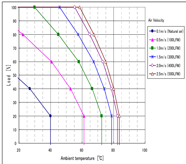
F-CBS-F3/F4 (H = 25.4mm)
