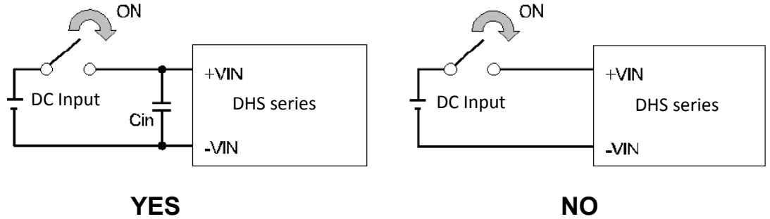
Fig. 2.2 External input capacitor
