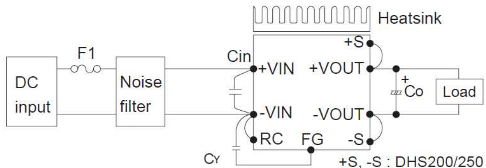
Fig. 3.1 Connection for standard use
