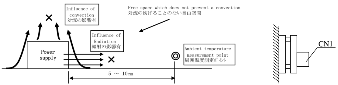
Mounting method(B)
