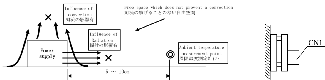
Mounting method(B)
